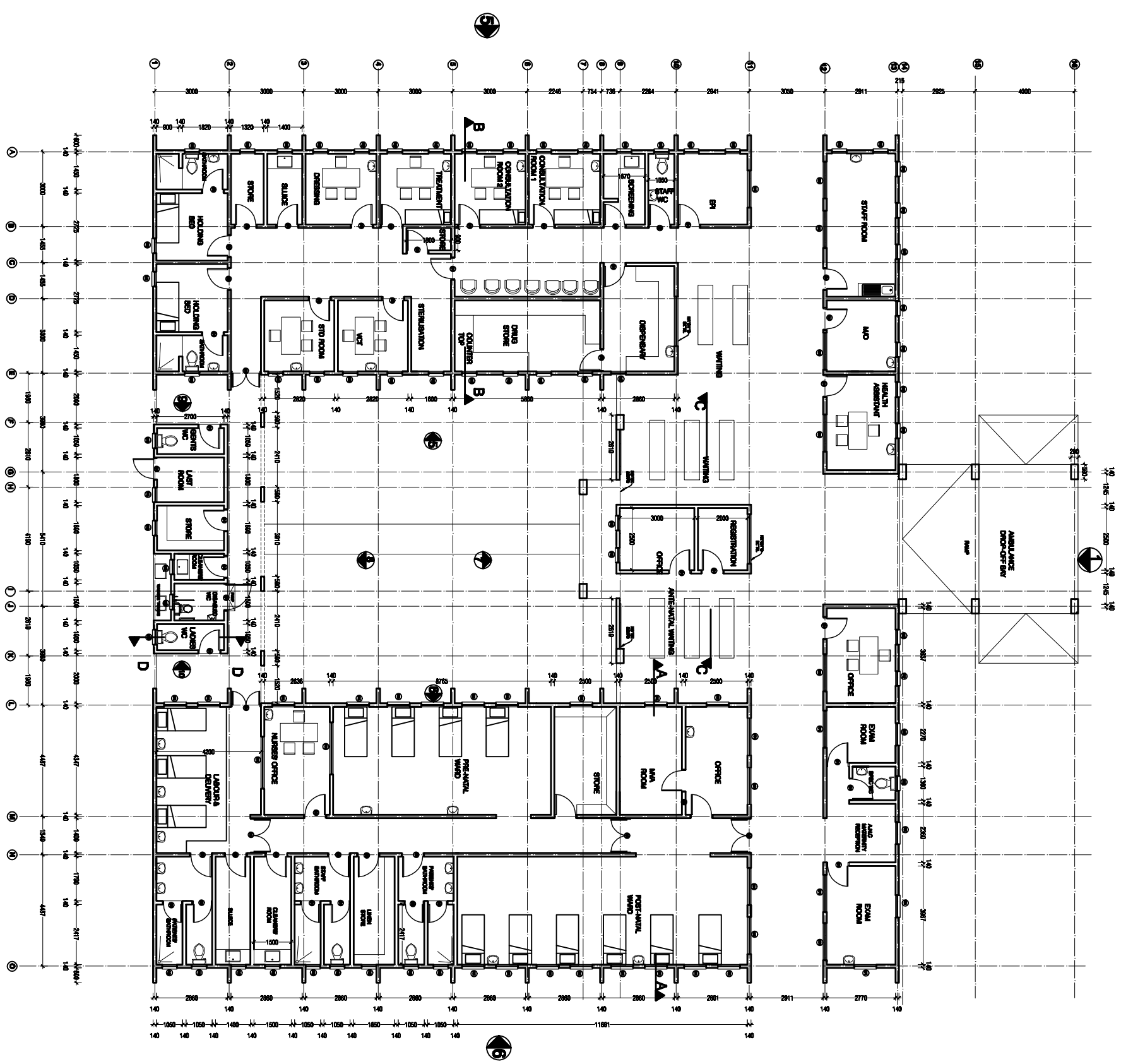
OPD FLOOR PLAN SCALE 1:100
